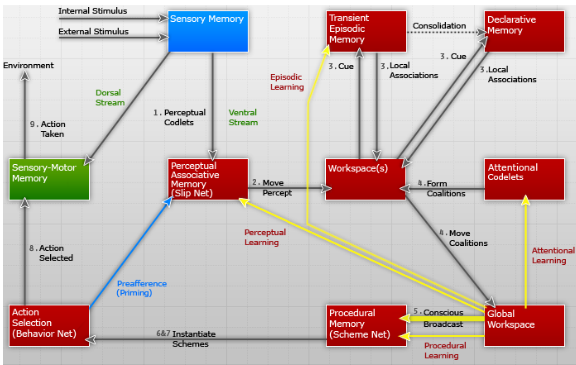
Figure 1. The LIDA Cognitive Cycle
